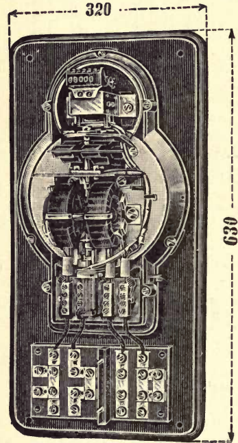
Fig. 280.—Interior of 30-Amp "Large Type" Oscillating Three-Wire Meter
